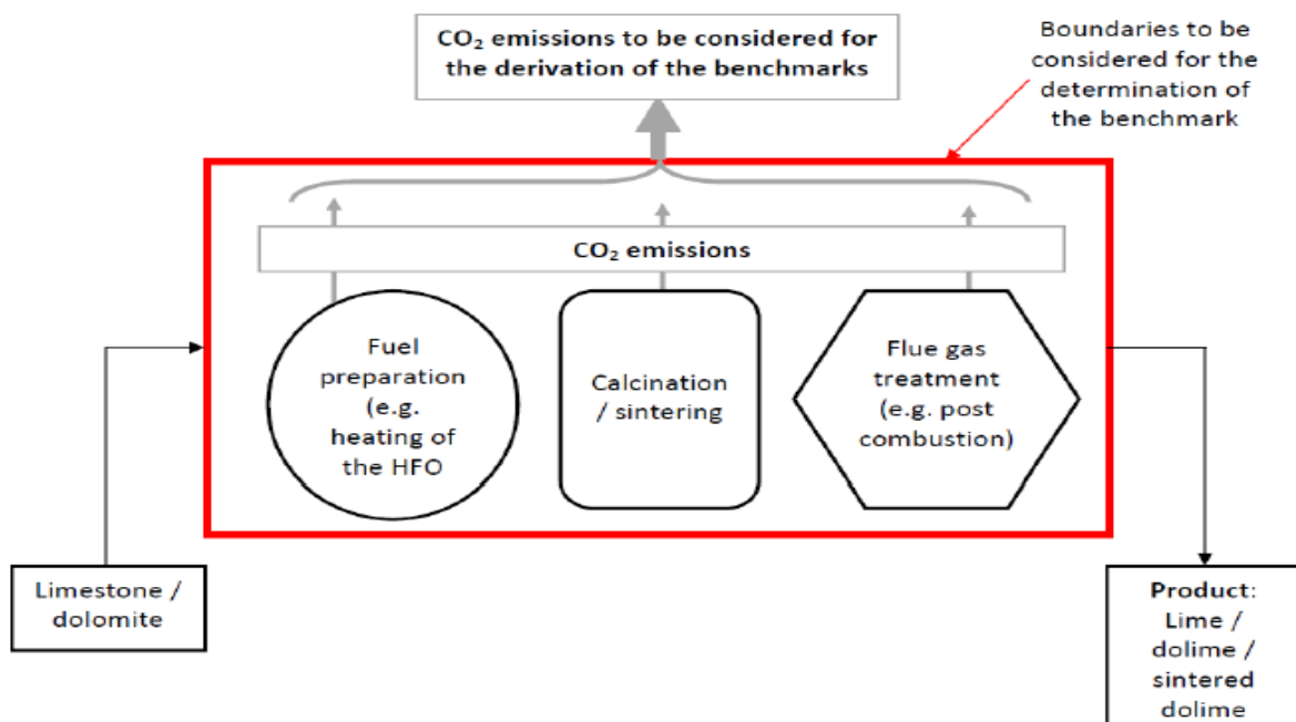
Figure 3. System boundaries (Sector Rule book for the development of CO 2 benchmarks for the European lime sector, 2010)
