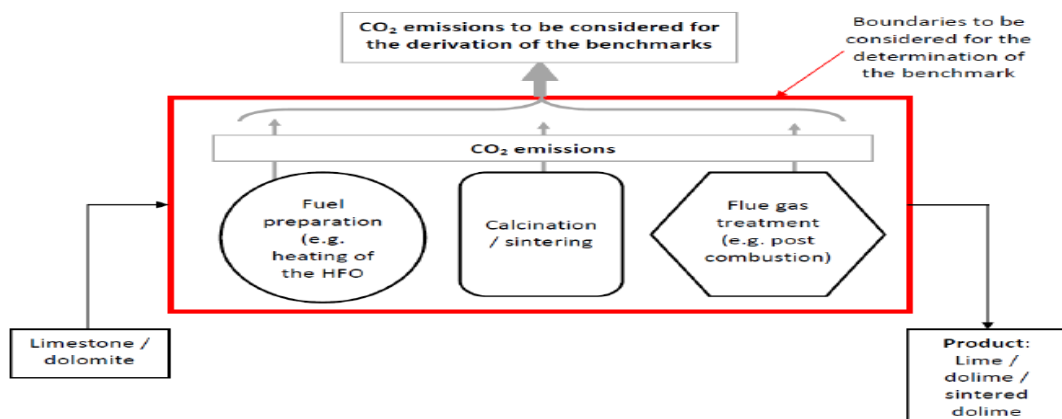
Figure 2. System boundaries (Sector Rule book for the development of CO 2 benchmarks for the European lime sector, 2010)
