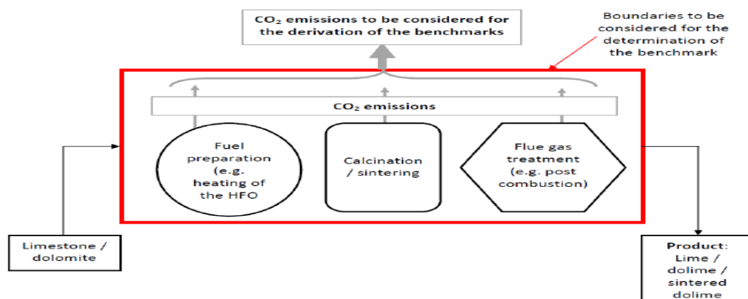
Figure 1. System boundaries (Sector Rule book for the development of CO 2 benchmarks for the European lime sector, 2010)
